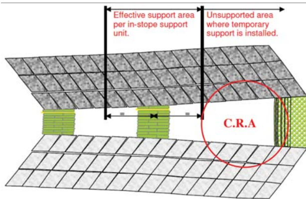
Figure 3—Diagrammatic section depicting the effect of a normal stope design
