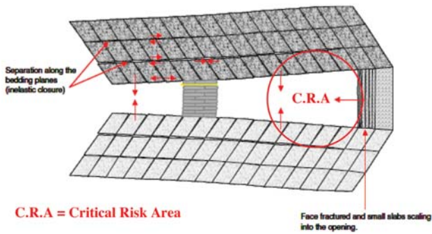
Figure 2—Sectional view showing typical stope closure
